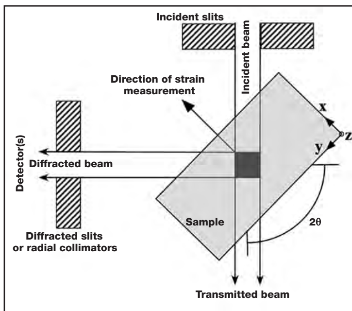
Fig. 4 — Schematic of neutron diffraction set up viewed from above shows nominal gauge volume (dark square) as defined by the slits [7] .
